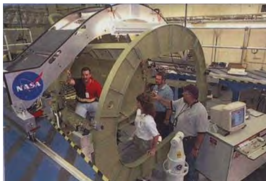
2000: The CRV X-38 rescue vehicle, controlled with a laser scanner from Unterentfelden/AG. ((RE41))
